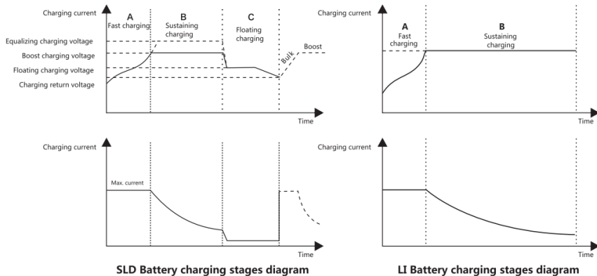
SLD Battery charging stages diagram
